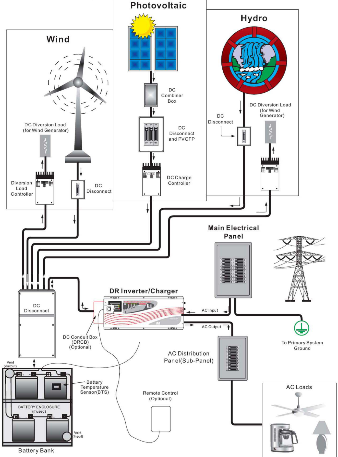
On-Grid Configuration - with Renewable Energy Sources
